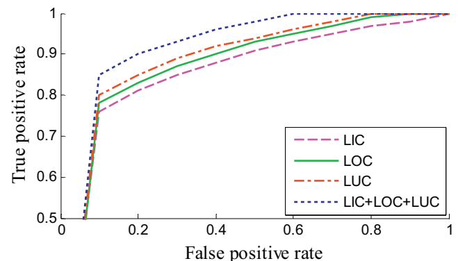
Fig. 8 – Classification performance of the descriptors proposed for cancer detection in terms of ROC curve.
