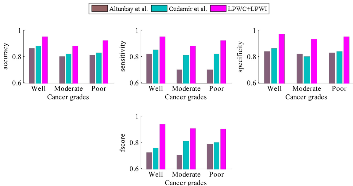
Fig. 16 – Performance comparison of the cancer grading phase of the proposed CCD system with existing cancer grading technique.
