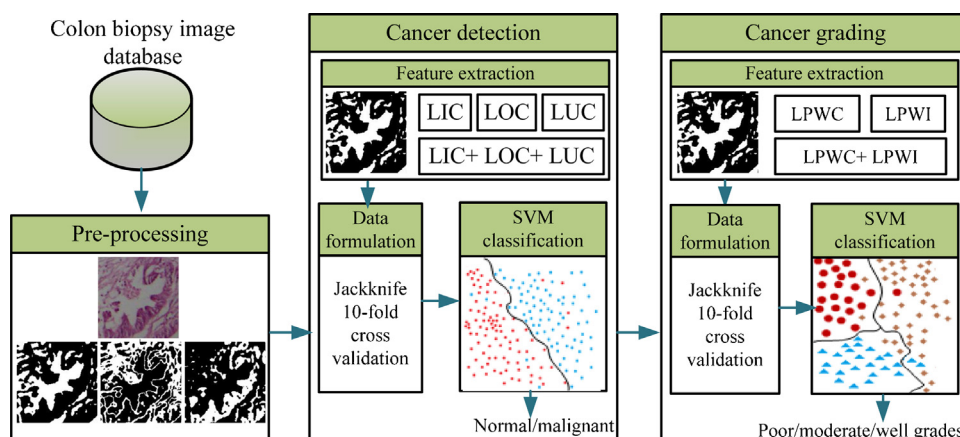
Fig. 2 – Schematic overview of the proposed CCD system comprising preprocessing, cancer detection, and cancer grading phases.
