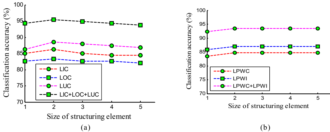
Fig. 7 – Classification performance of the proposed individual and hybrid descriptors as a function of \alpha : (a) cancer detection and (b) grading phases.
