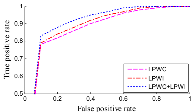
Fig. 11 – Classification performance of the descriptors proposed for cancer grading in terms of ROC curve.
